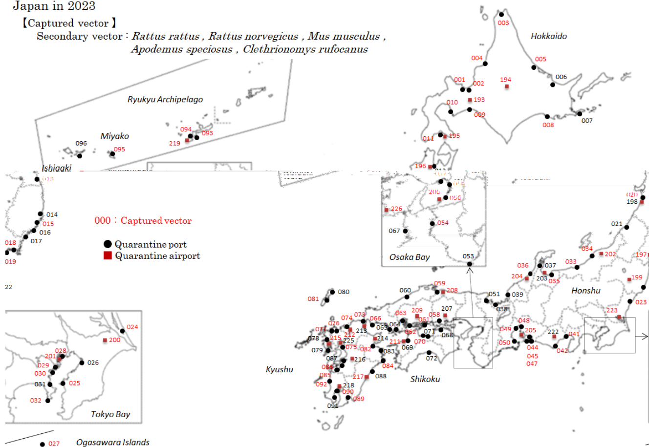
Figure 9 Vector situations of hemorrhagic fever with renal syndrome at quarantine ports and airports, Japan in 2023
